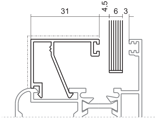
1967 0.349 Kg/m
