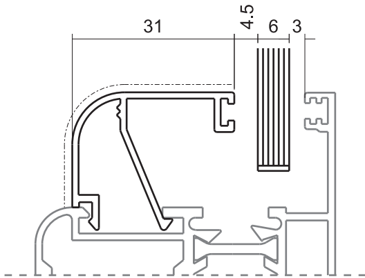
1961 0.327 Kg/m
