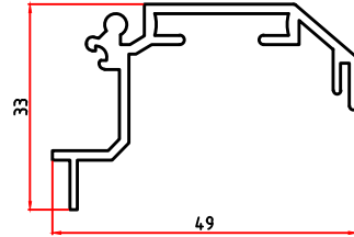
2870 0,544 Kg/m ( 2869-3959-4131 )
