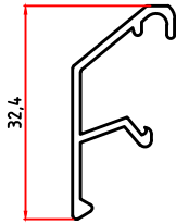
2869 0,215 Kg/m ( 2870 )
