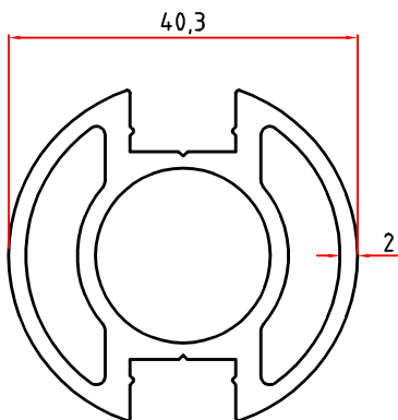
2646 1,225 Kg/m
