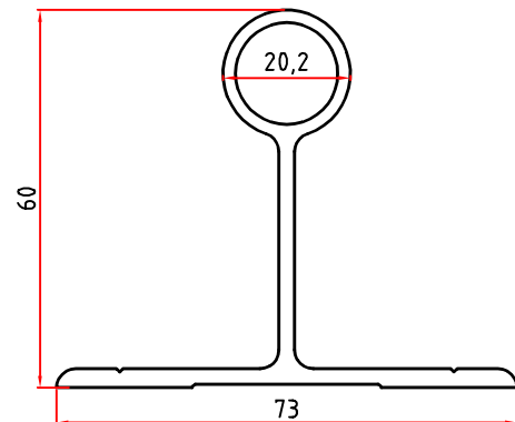
4887 1,172 Kg/m
