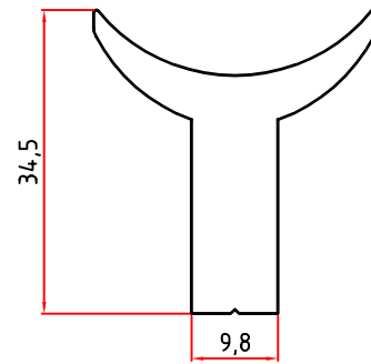
2767 1,056 Kg/m
